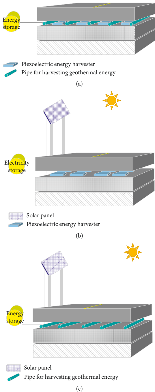
FIGURE 8: Hybrid energy harvesting systems: (a) hybrid piezo-electric-thermoelectric energy harvester, (b) solar-piezoelectric composite energy harvester, and (c) solar-geothermal energy harvester (based on [88]).
